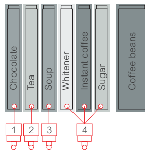
Variant 6402 1 large bean container 6 instant product containers, 4 mixer units
