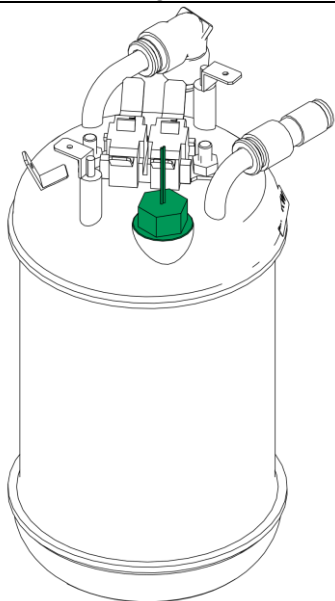
Previous boiler with temperature sensor with integrated screw-in fitting
