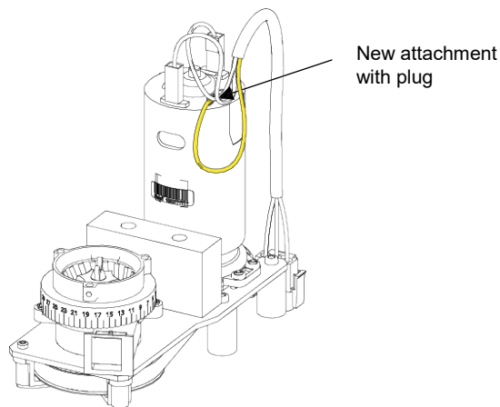
New built-in grinder
