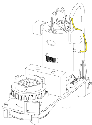
Previous built-in grinder
