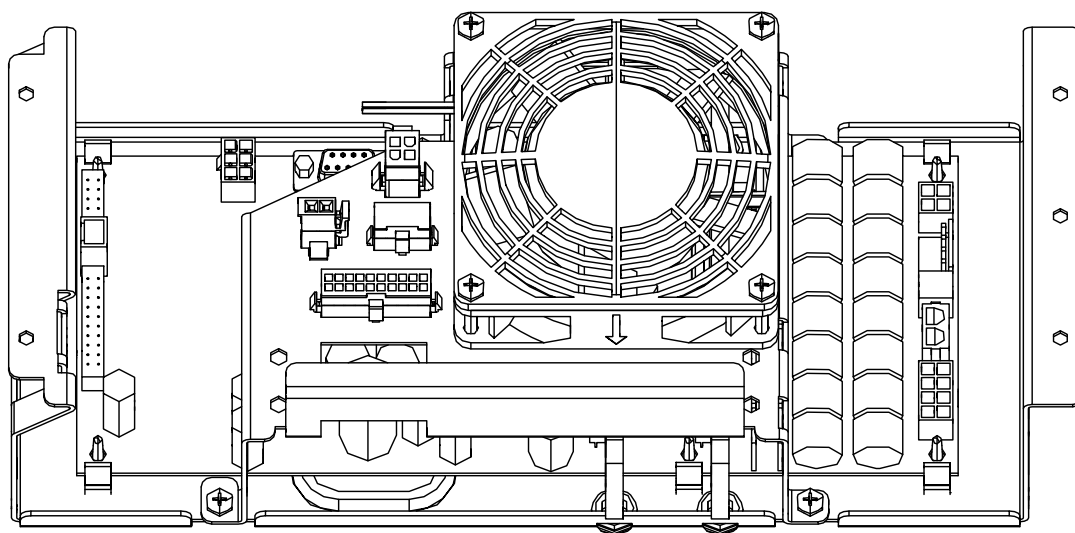
7010430700 Control board holder compl. assembled IMAX 2 microstep driver
