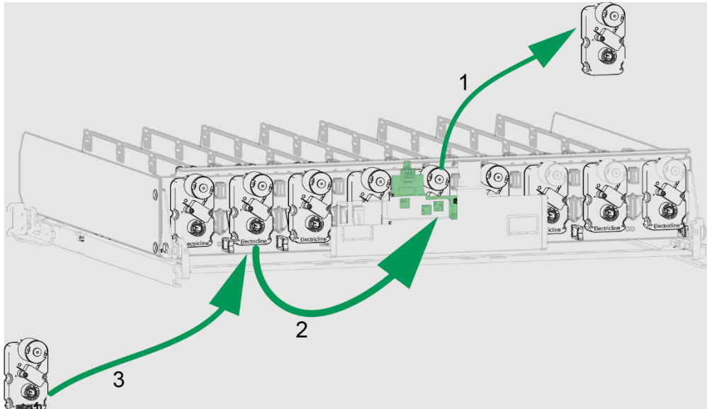
Figure 1 Goods compartment with ElectricLine motors - Bitron motor as a new spare part
